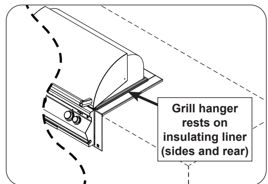
Fig. 4-2 Install grill into liner
