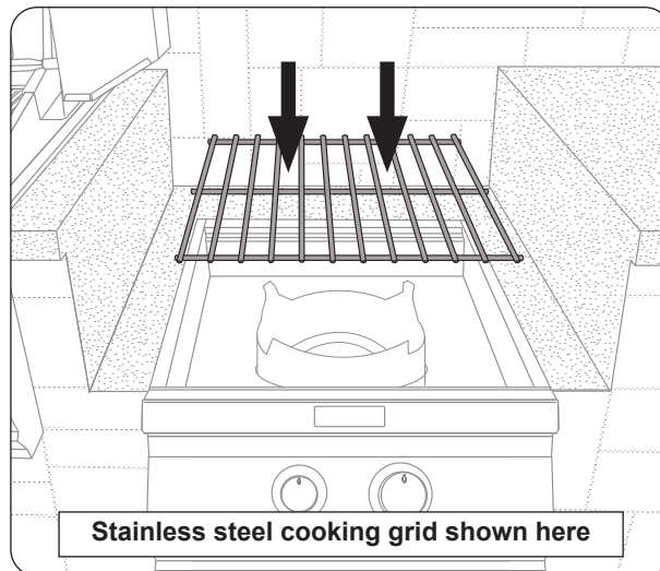
Fig. 25-4 Install cooking grid
