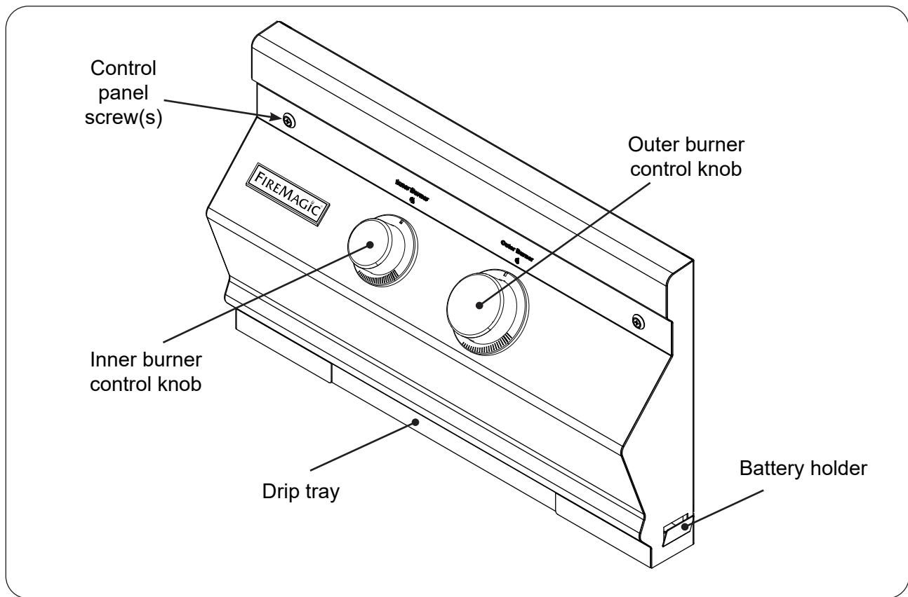
Fig. 27-1 Power burner controls
