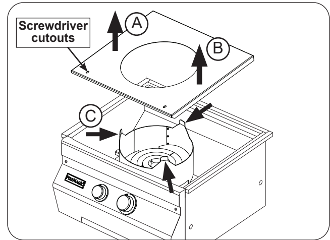
Fig. 34-1 Interior protection plate removal
